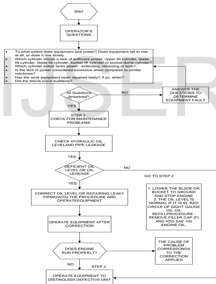
Figure 1: Failure mode algorithm flowchart
